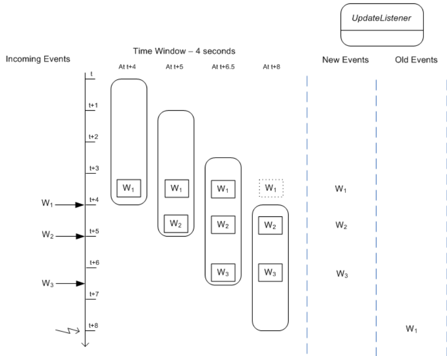
Figure 3.5. Output example for a statement with a time window
